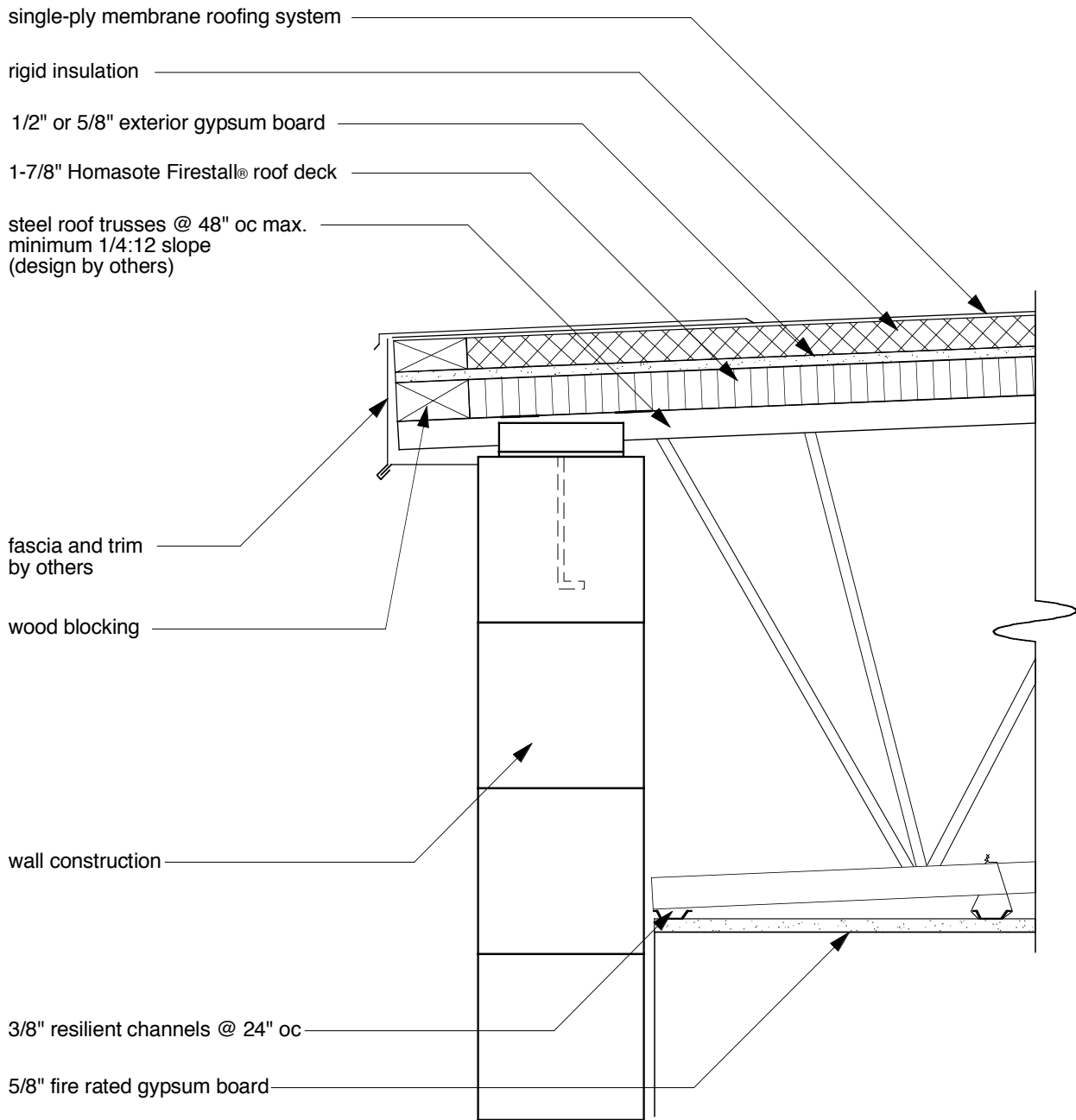
Firestall® Roof Deck Detail FS-SP-ID-178-48-26 UL Design No. P535
