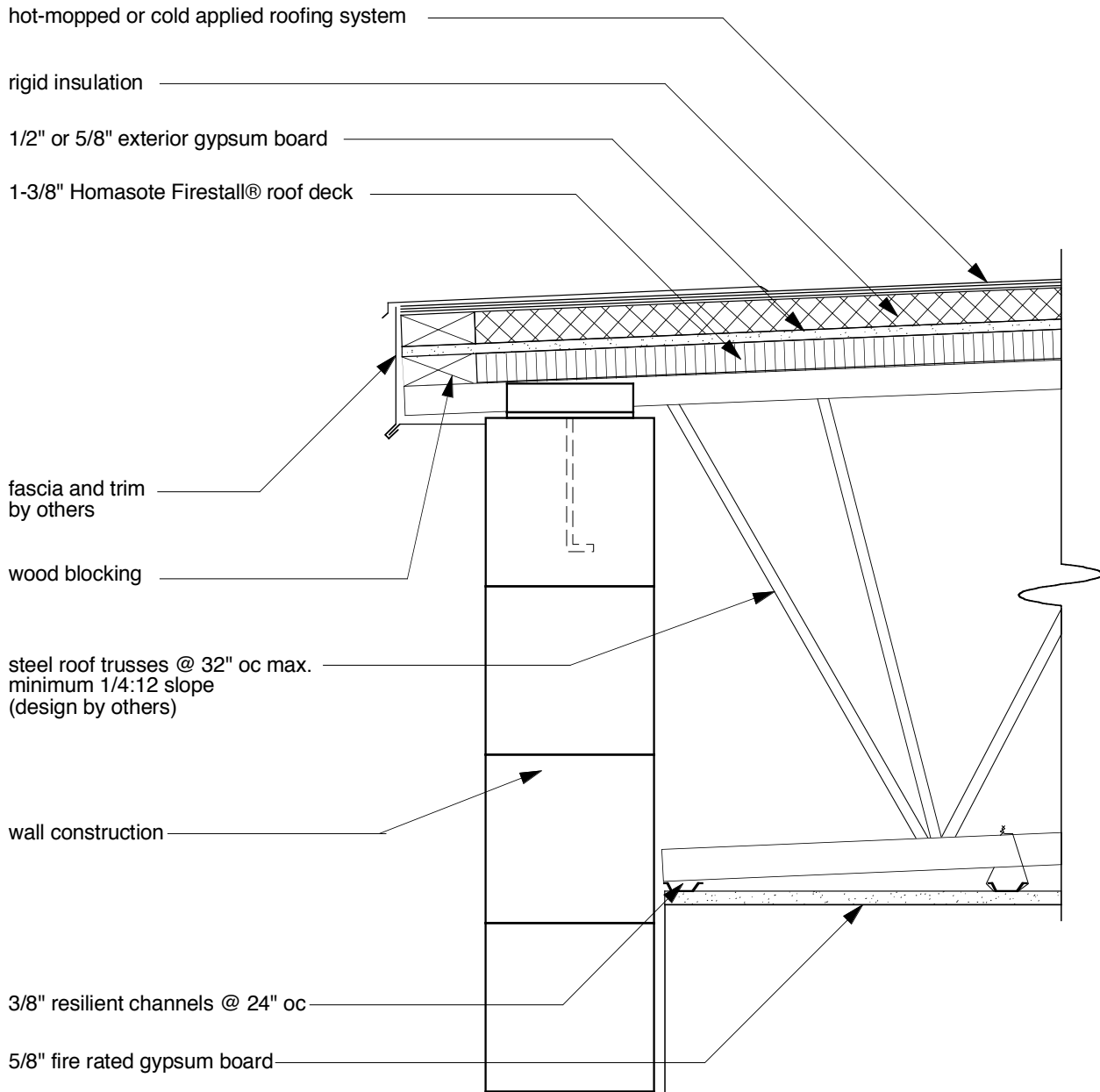
Firestall® Roof Deck Detail FS-HMCA-ID-138-32-13 UL Design No. P535
