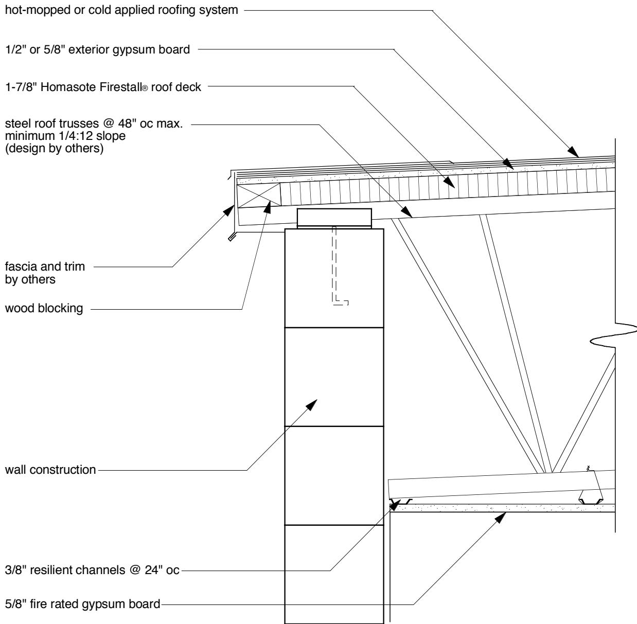
Firestall® Roof Deck Detail FS-HMCA-GBO-178-48-21 UL Design No. P535
