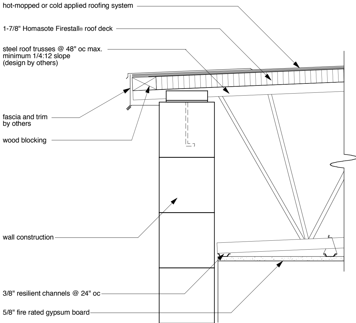
Firestall® Roof Deck Detail FS-HMCA-178-48-17 UL Design No. P535
